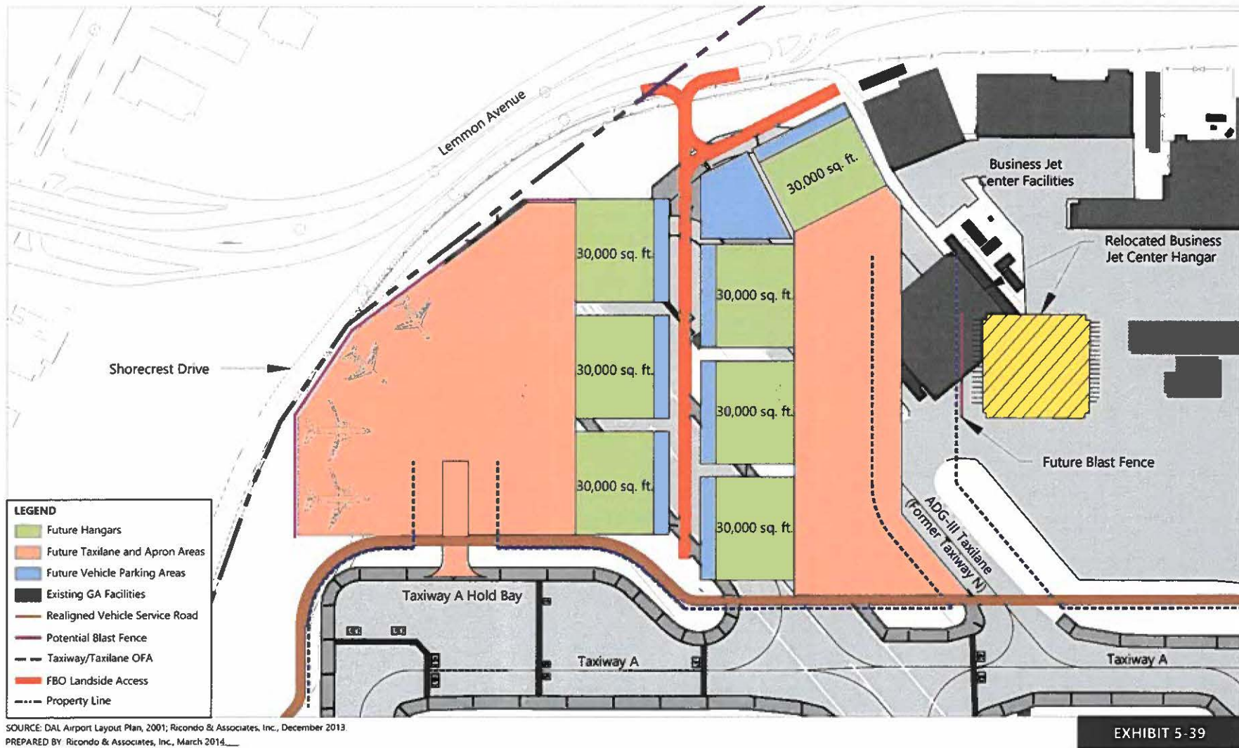
North Corner General Aviation Facility Layout Alternative 1C
