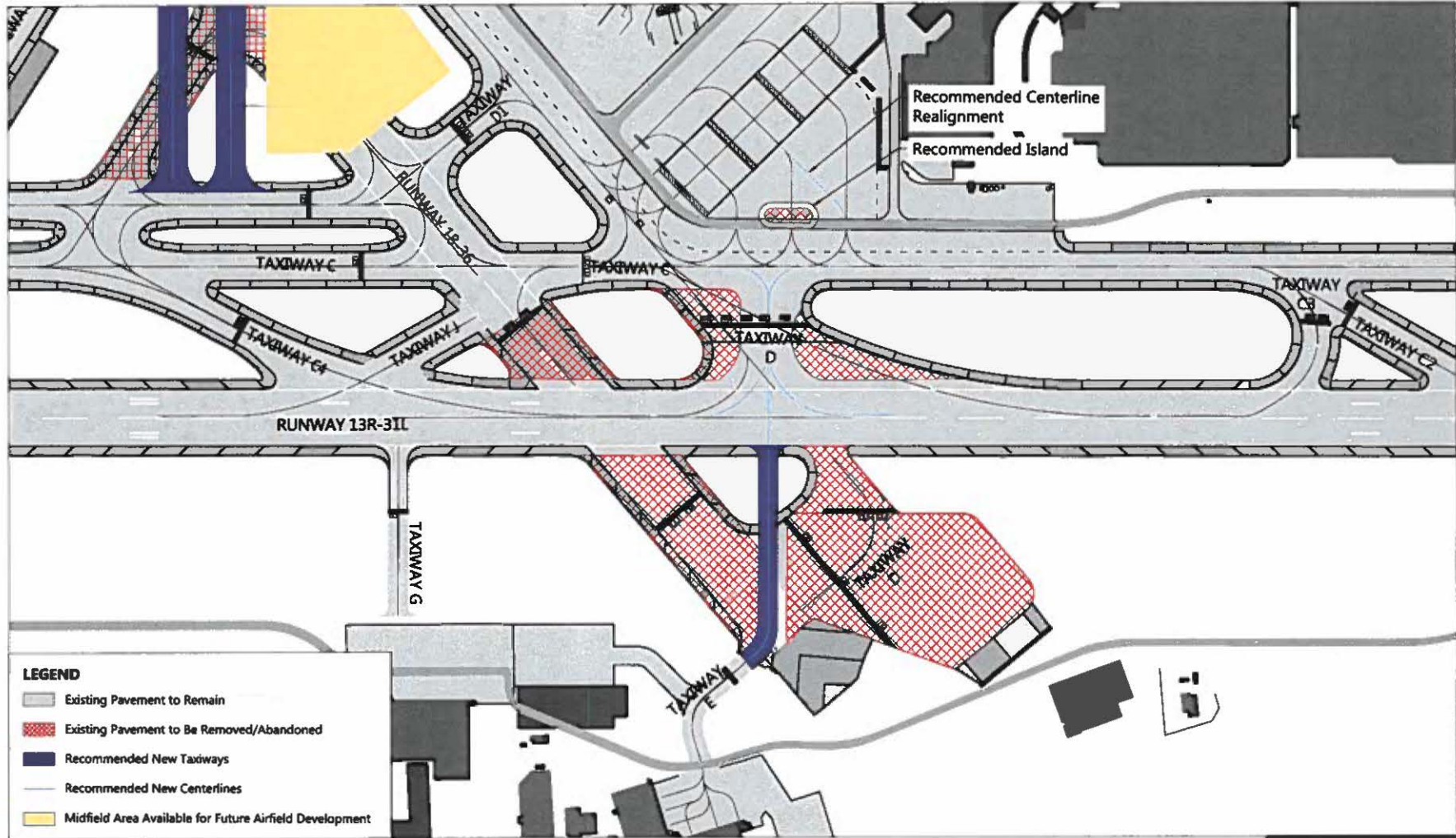
Modifications to Taxiway D Crossing of Runway 13R-31L with Runway 18-36 Decommissioned
