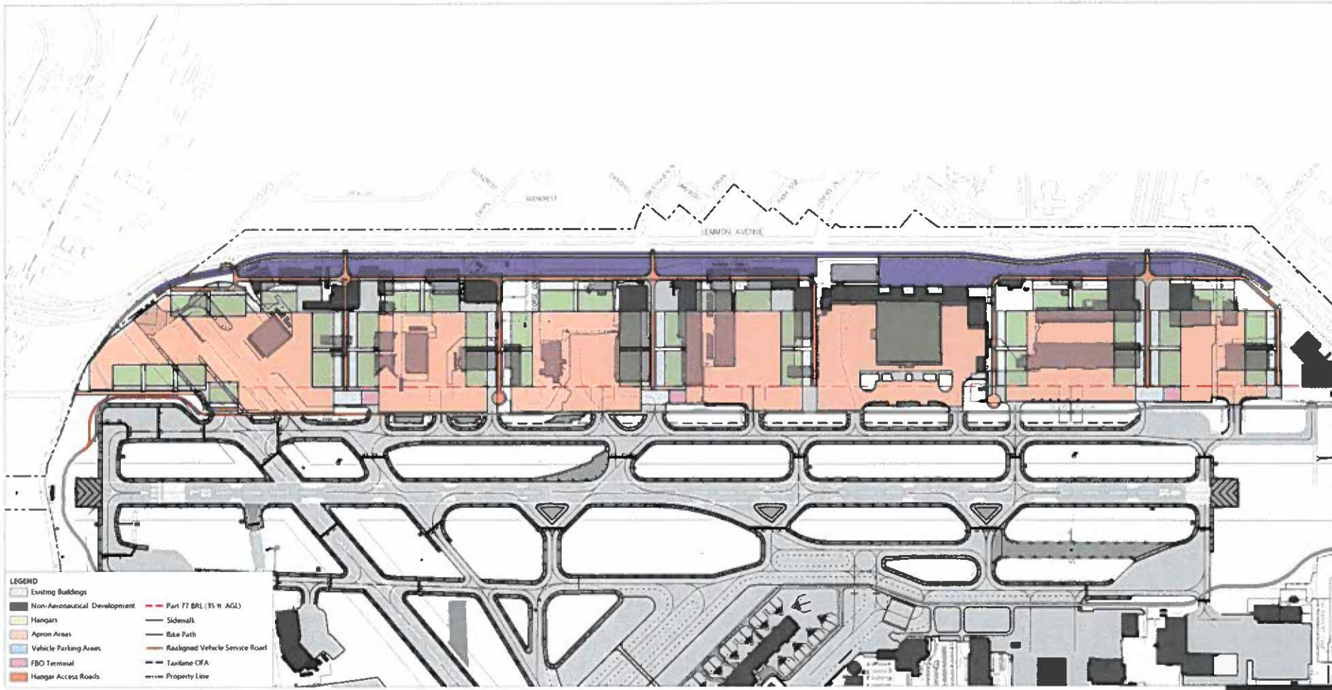
Lemmon Avenue Redevelopment Alternative 3A with Runway 18-36 Decommissioned
