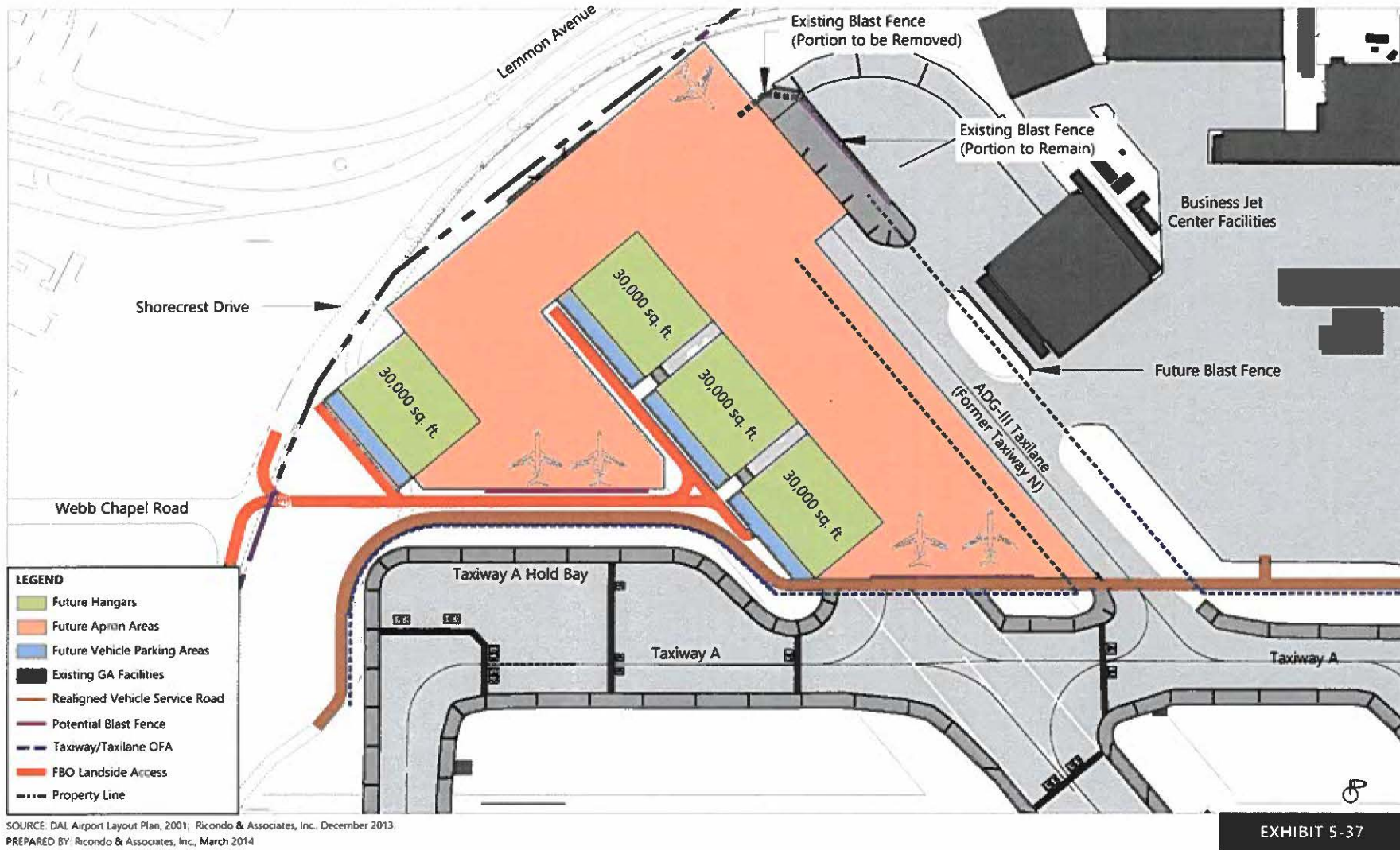
North Corner General Aviation Facility Layout Alternative 1A
